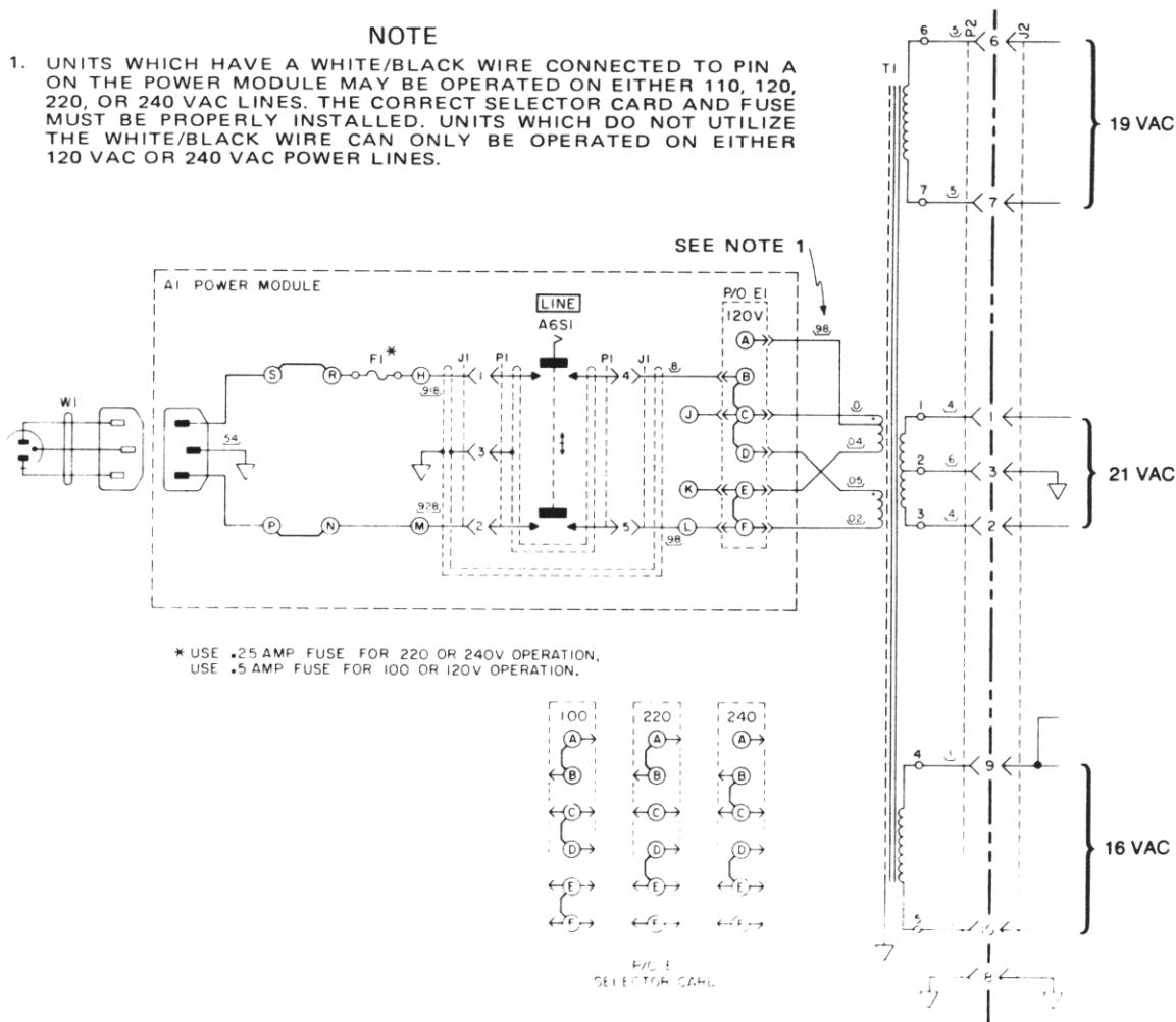
Figure 5-1. Primary Power Schematic
