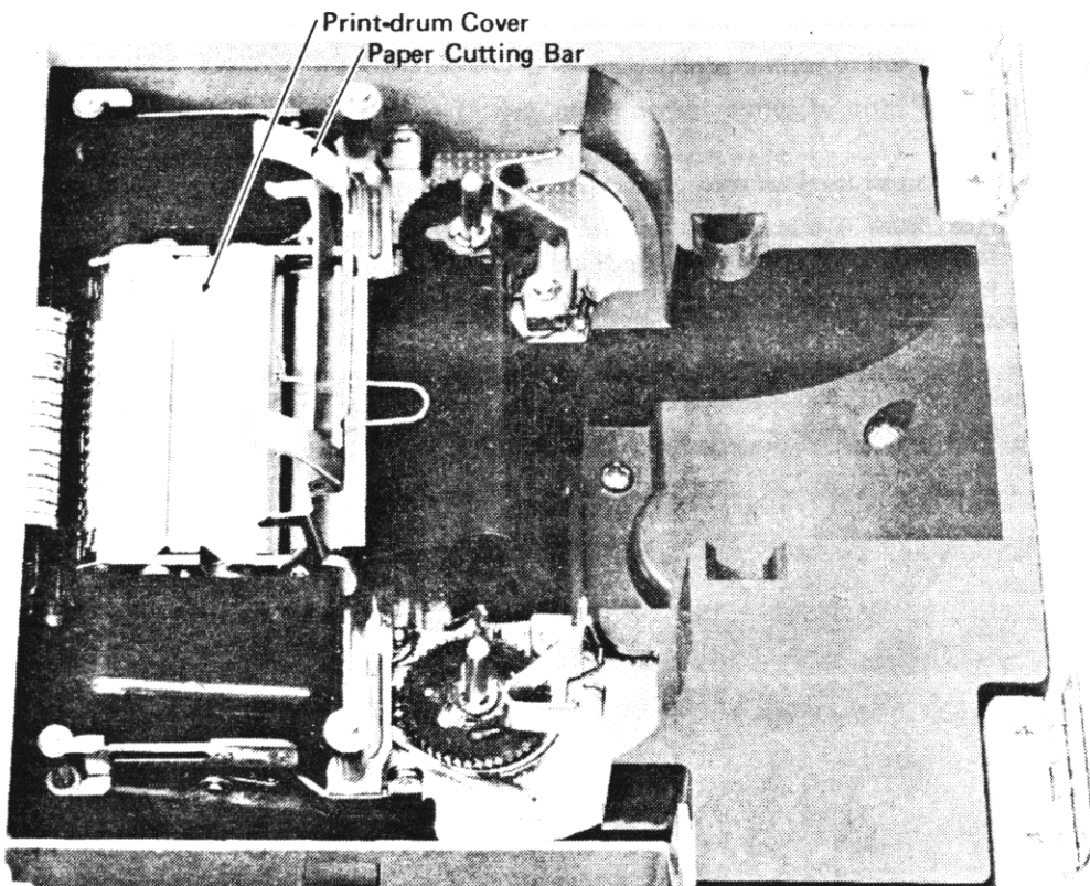
Figure 3-1. The Cutting Bar and Print-drum Cover.
